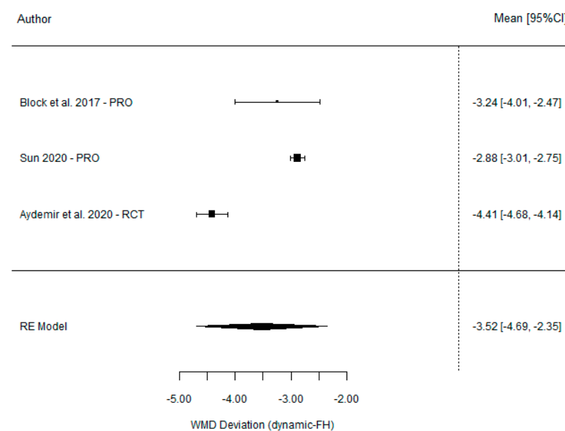
Figure 6. Forest plot illustration of the angular deviation (comparison between DGS and FH).
